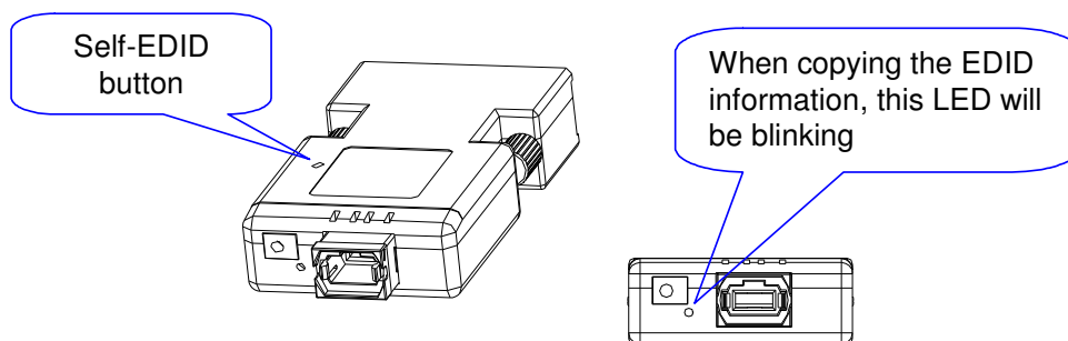
Figure 3 self-EDID Mode
